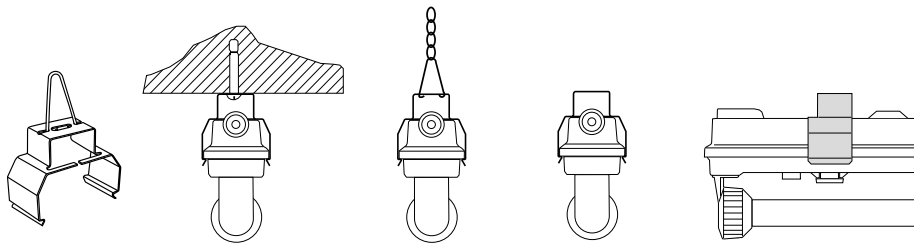
Mounting Kit
